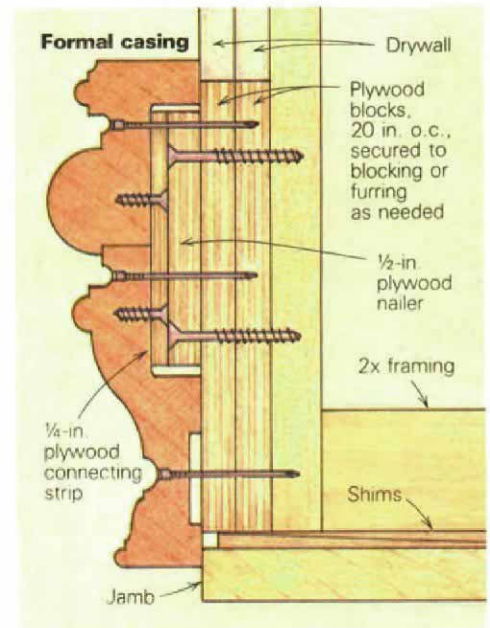
To anchor the formal casings, plywood blocks, seen on the right edge of the door in the photo below, were screwed to the stud wall and the drywall was notched around them. A 1/2-in. plywood nailer was then screwed to the blocks to provide solid backing for the 7 1/2-in. wide door casings, as shown in the drawing at right.
